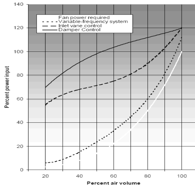
Figure 1 – Input Power versus Flow for a Ventilation Systems 2 . Example of the type of system curves that is necessary for calculations.
